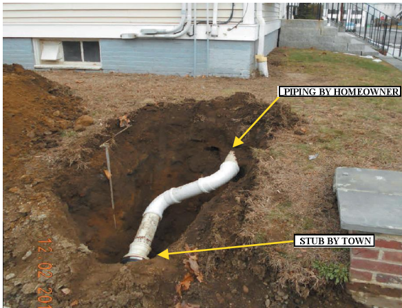
MUNICIPAL DRAIN SERVICES
