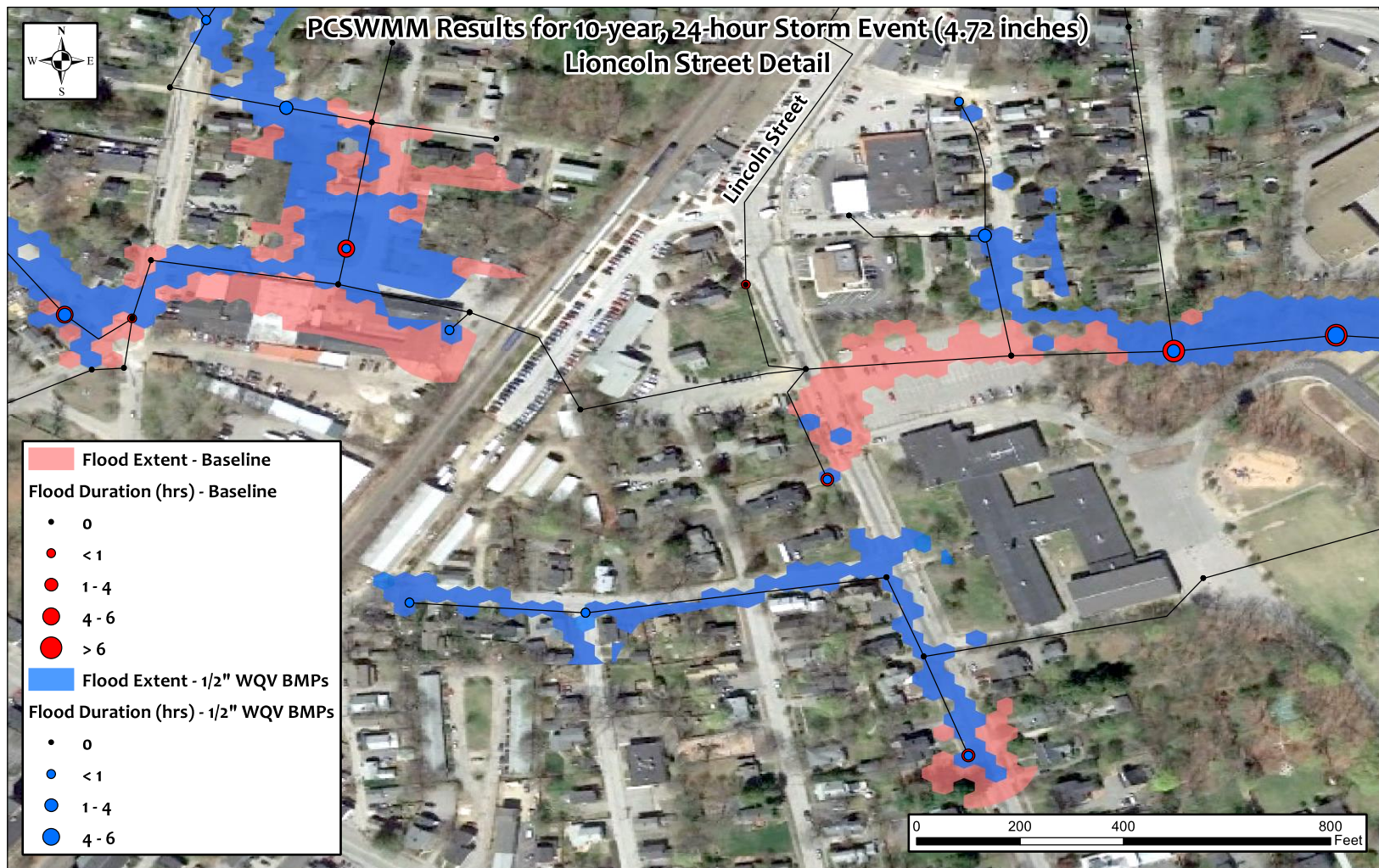
Figure 34: Modeled Flood Reduction Impacts of BMP 3 (sized for 1/2" WQV)
